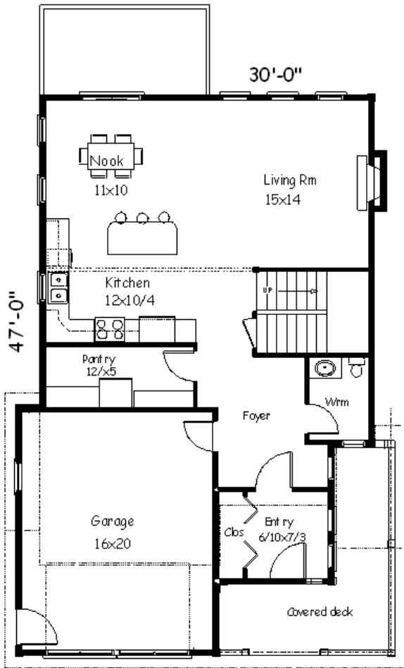
1st FLOOR PLAN 900 sq ft
