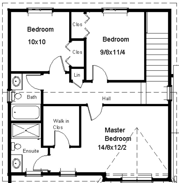
2nd FLOOR PLAN 780 sq ft
